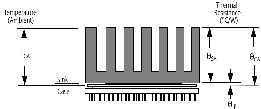
Figure 91. Thermal Model
